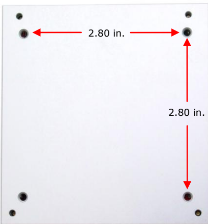
Aurora's aluminum thermal dissipation heatspreader with standardized mounting hole pattern
